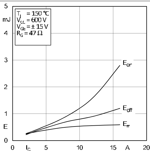
Fig. 3: Typ. turn-on /-off energy = f(I_D)
